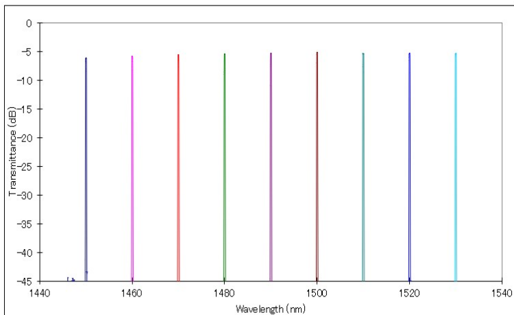
Filter Wavelength Tuning Range
