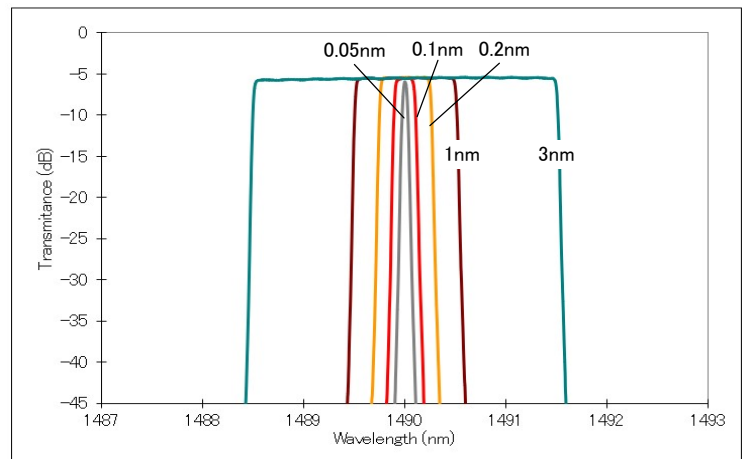
Filter Spectra at Various 3dB Bandwidth
