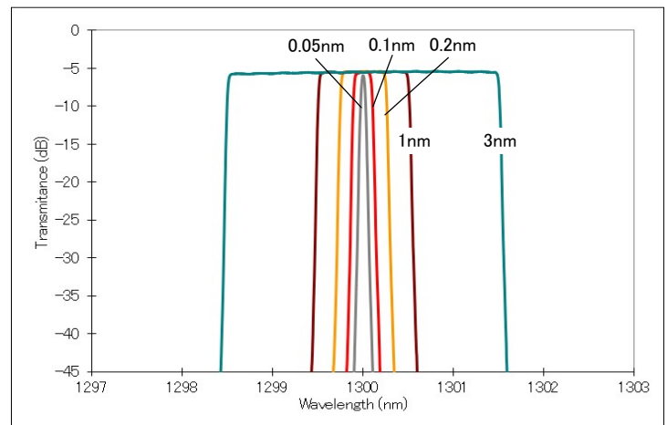
Filter Spectra at Various 3dB Bandwidth
