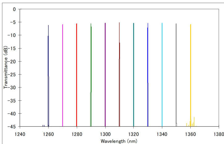
Filter Wavelength Tuning Range
